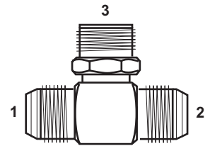
F6803-NWO FO-FO-MAORB TEE
