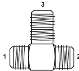
2703 MJ-MJ-MJ BULKHEAD BRANCH TEE
